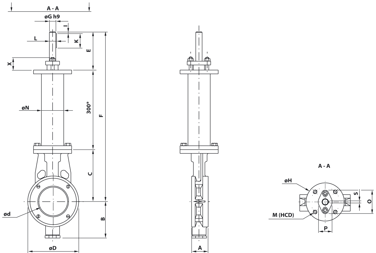
Butterfly valve, type VSS LT (Low Temperature)
