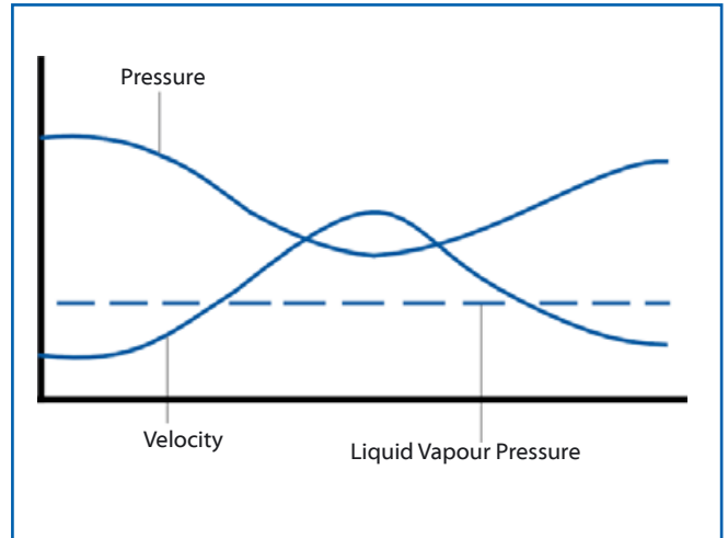
Fig. 2: Pressure and velocity variations with noise reduction trim. Compare with Fig. 1.
